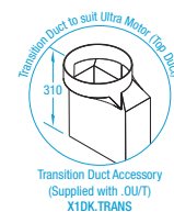
Ultra Motor Outlet 226mm x 97mm
