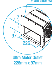
Transition Duct Accessory (Supplied with .OU/T) X1DK.TRANS
